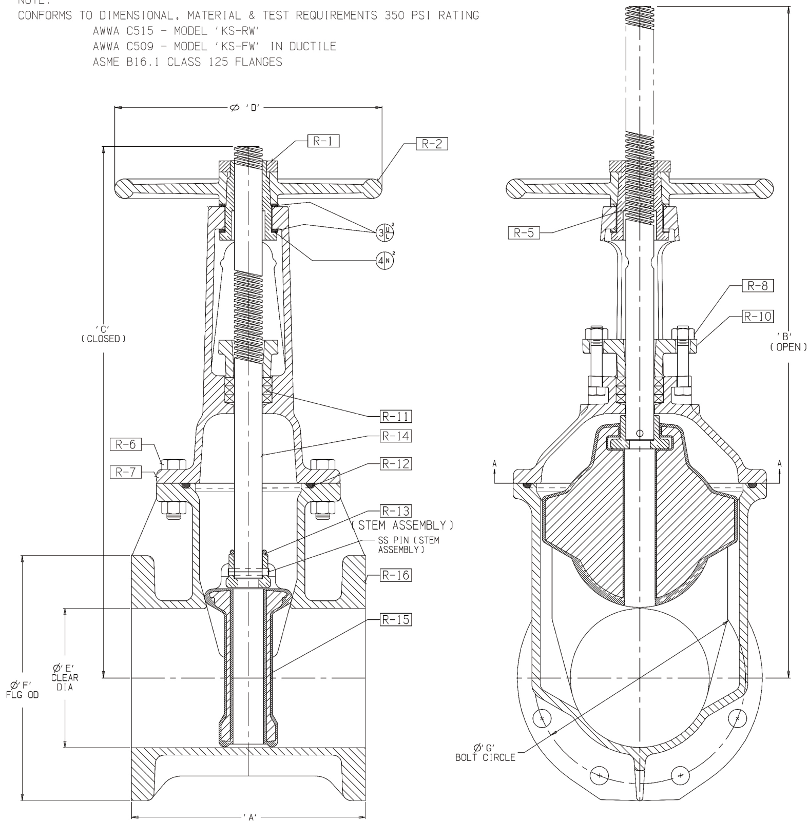
ALL FLANGE VALVES TAPPED & PLUGGED @ POSITION "A"
